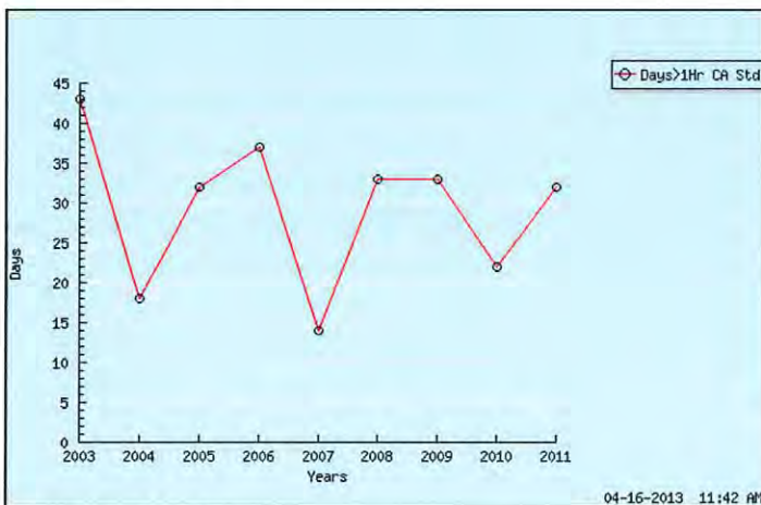
Figure 3 - PM 10 Data
