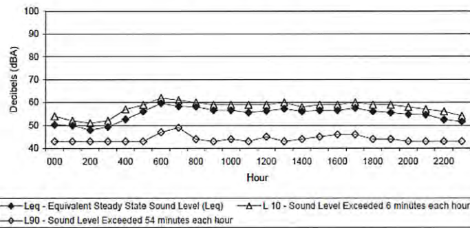
Figure 8 - Noise Measurement
