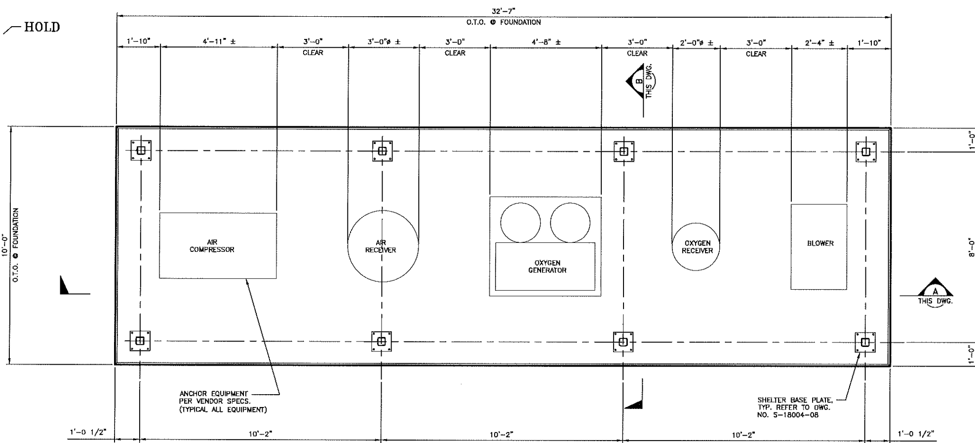
FOUNDATION PLAN SCALE: 1/2"=1'-0"
